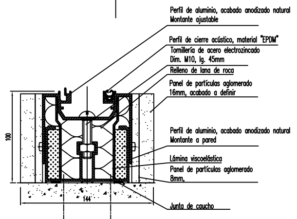
DETALLE PAL
